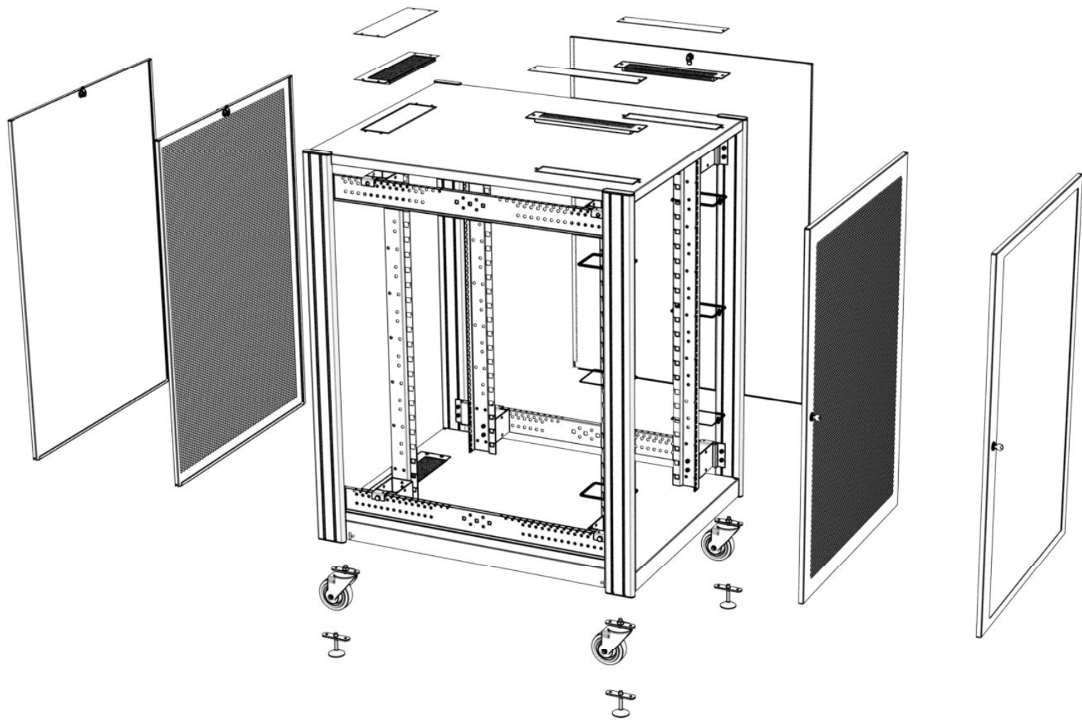
Omara 19" ServerM, širina 800mm
