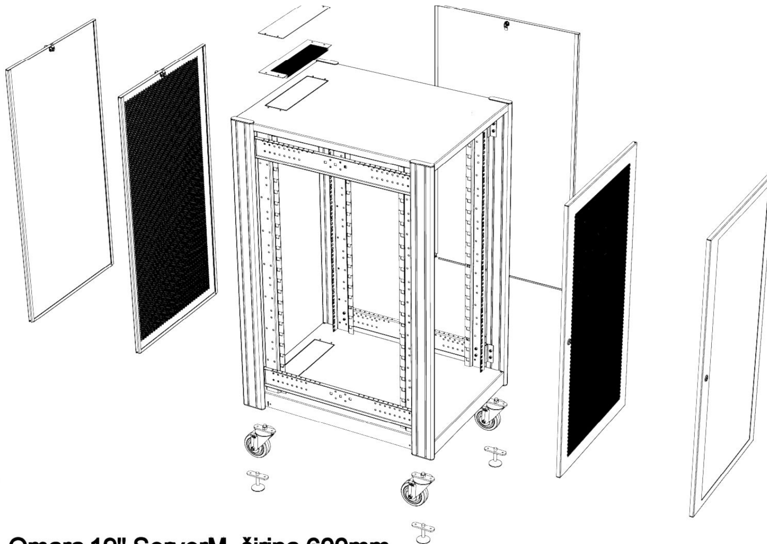
Omara 19" ServerM, širina 600mm
